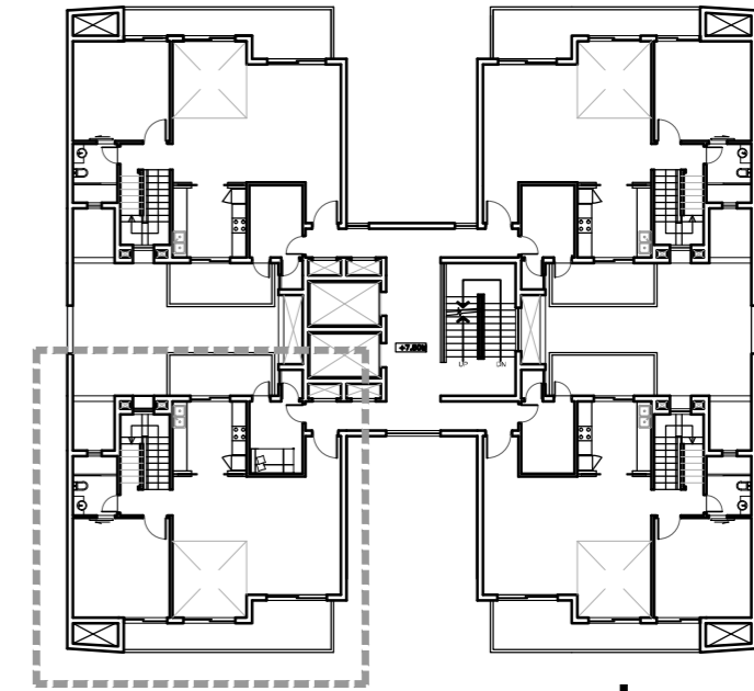
key plan
